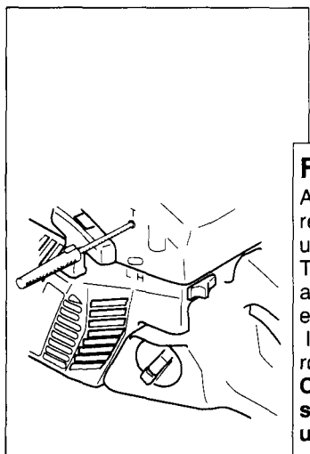
CARBURETOR MIXTURE NEEDLES WITH LIMITER CAPS
