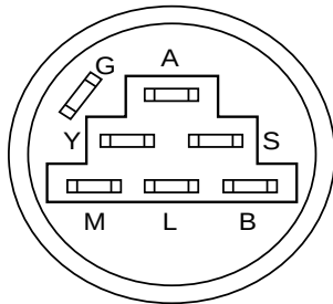
IGNITION SWITCH
