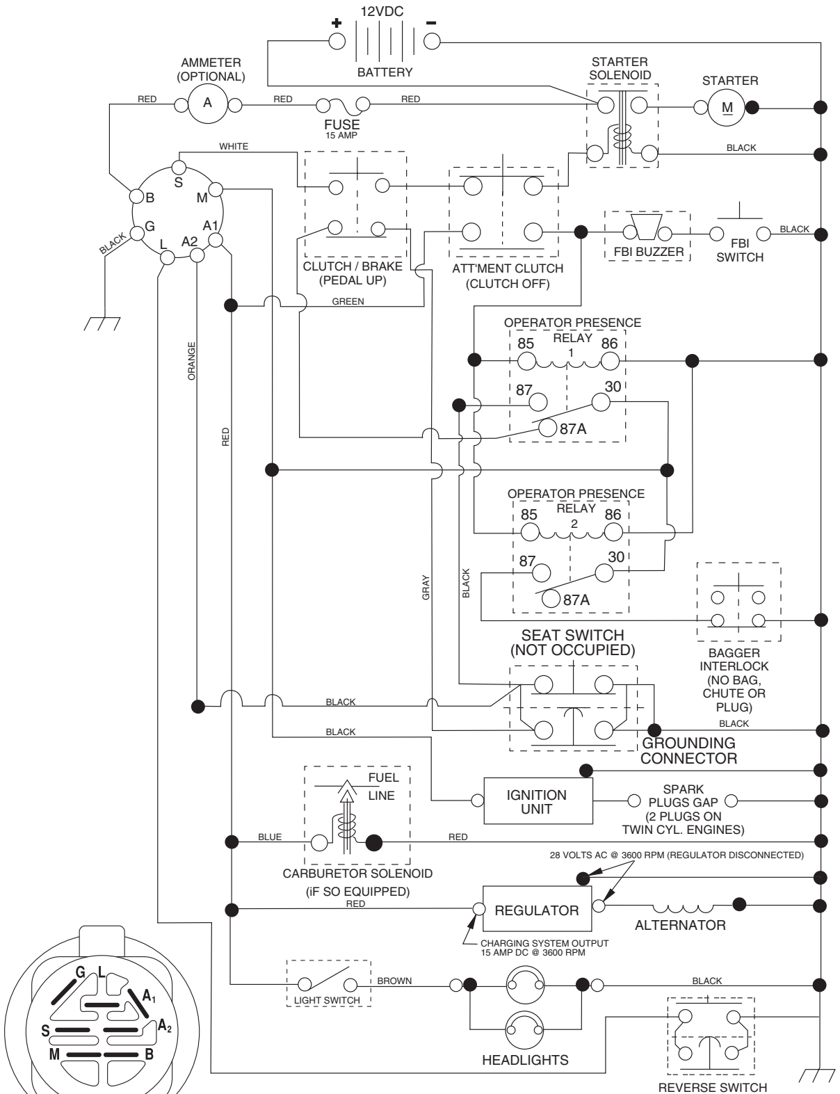
IGNITION SWITCH
