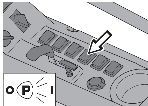
Parkeringsljus
