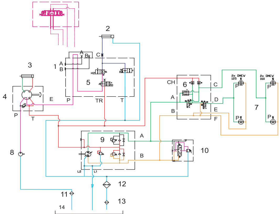
Hydraulschema
