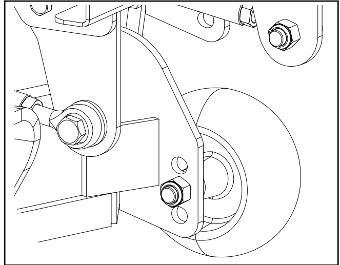
Anti-scalp rollers
