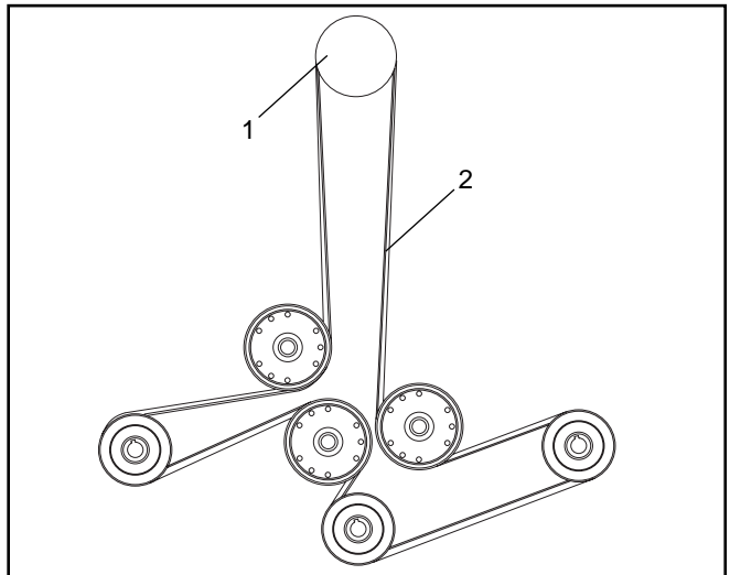
1. Clutch pulley 2. Deck belt Belt routing, deck belt
