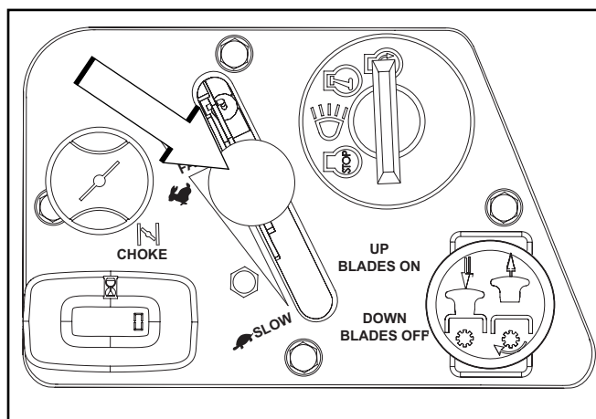
Throttle control
