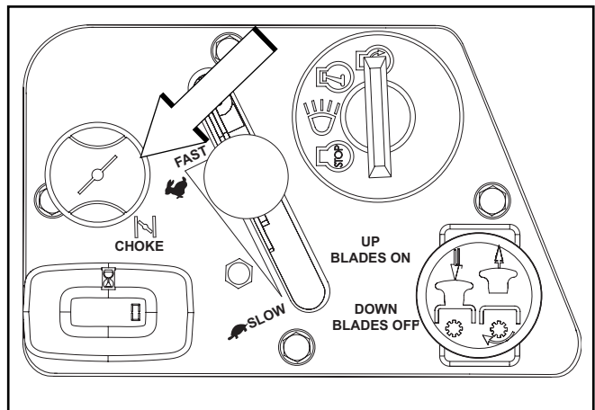
Choke control
