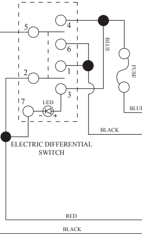
ELECTRIC DIFFERENTIAL SWITCH CONNECTOR
