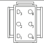
CHASSIS HARNESS CONNECTOR (MATING SIDE)
