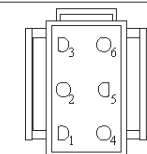
CHASSIS HARNES CONNECTOR (MATING SIDE)
