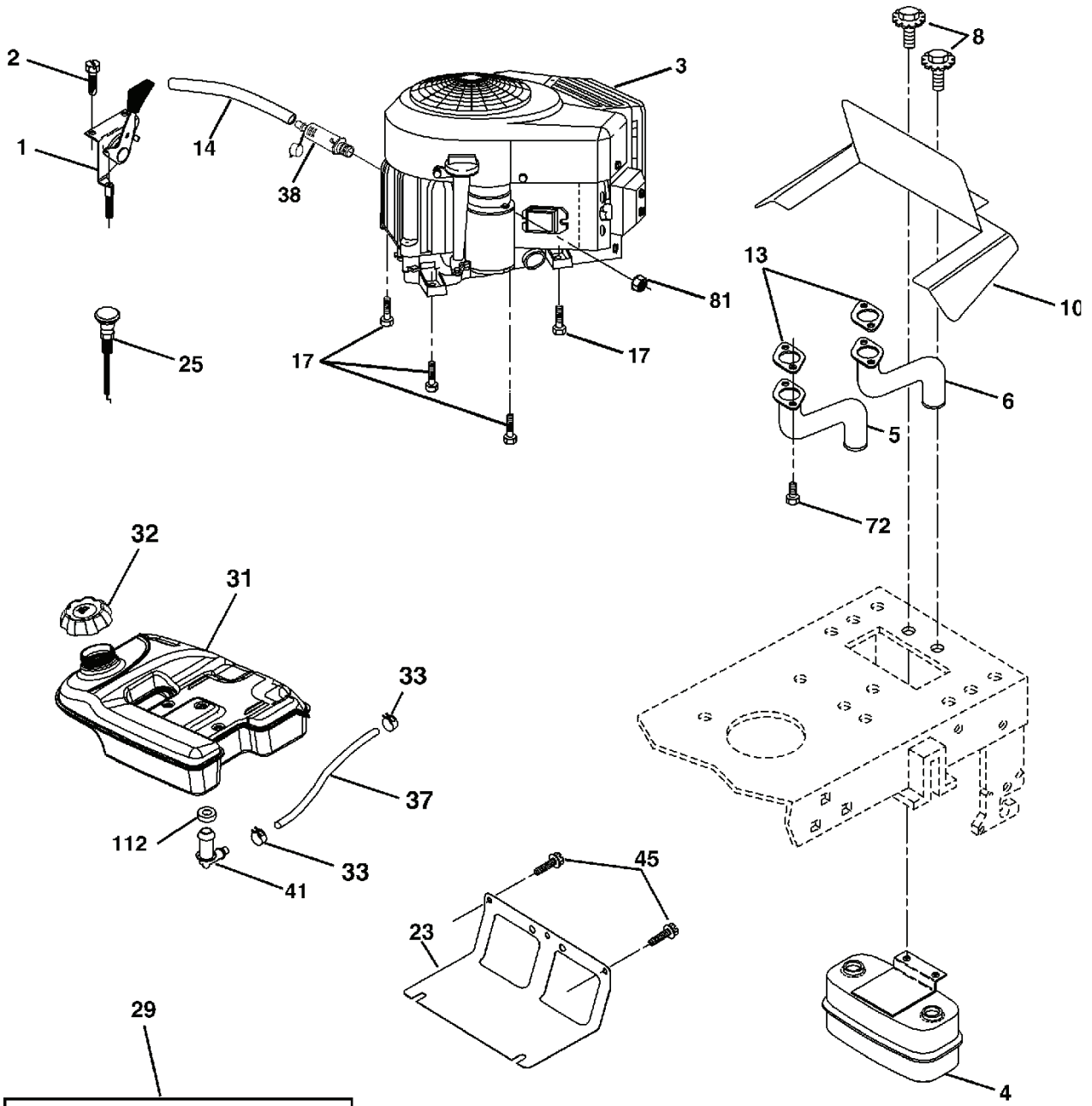
OPTIONAL EQUIPMENT Spark Arrester
