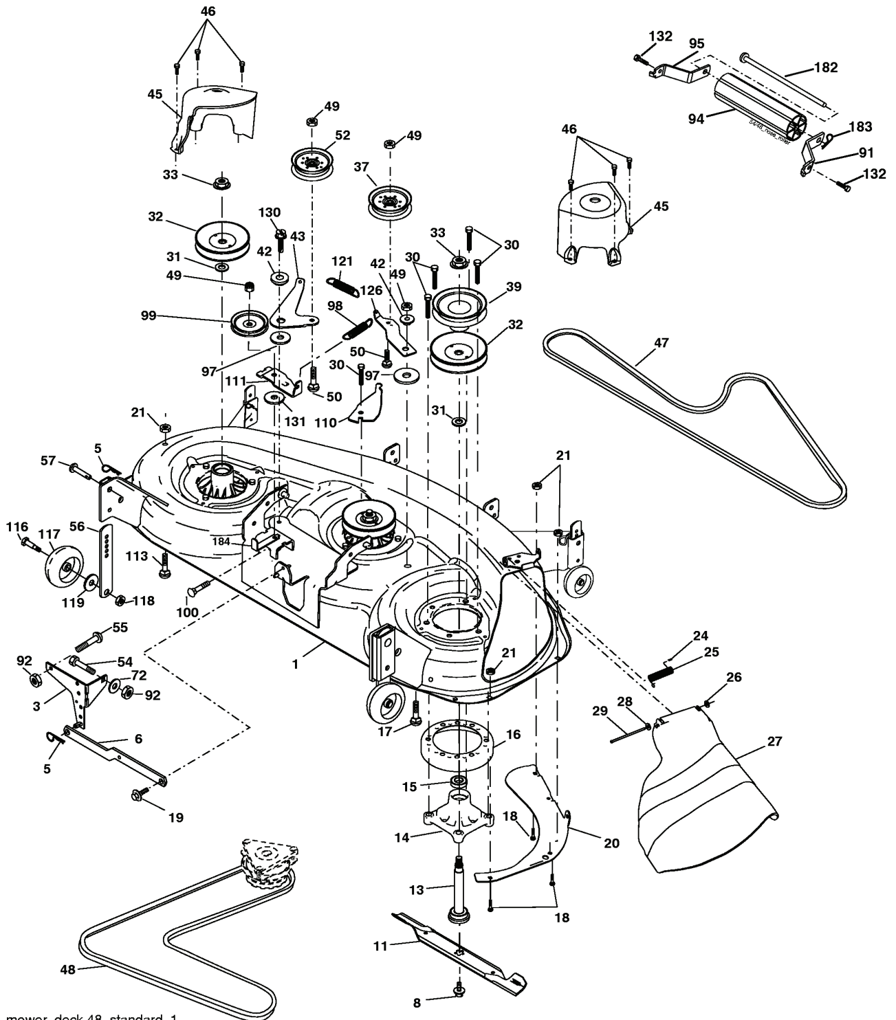
mower_deck.48_standard_1
